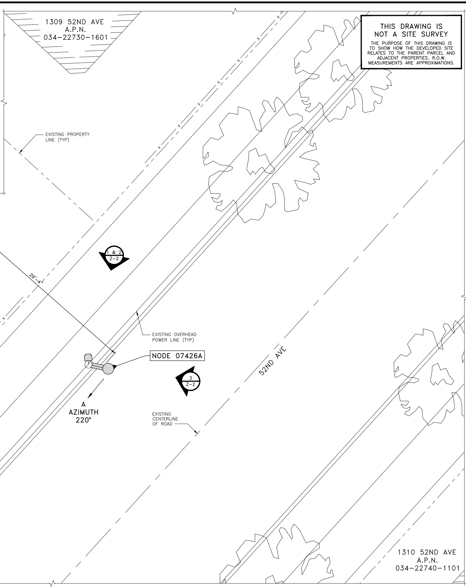
OVERALL SITE PLAN
