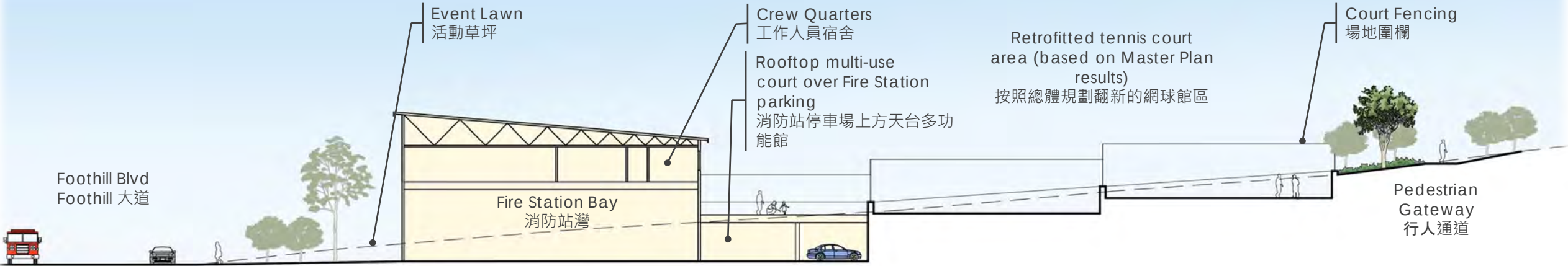
North-South Section | 南北剖面圖
