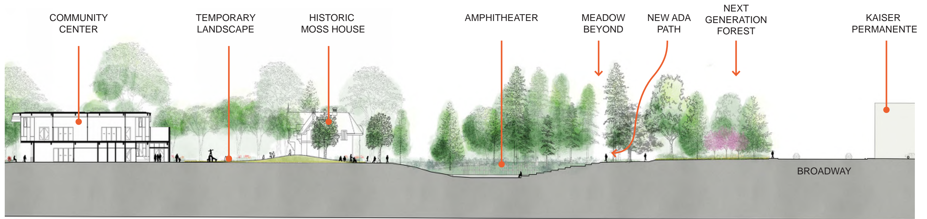
East - West Section Of Amphitheater
